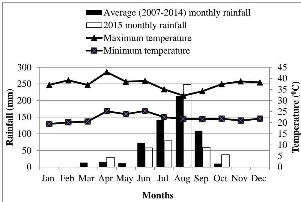
Fig. 2. Average (2007-2014) and 2015 Monthly Rainfall Amounts (mm) and Distributions in a Year and Average (2008-2011) Monthly Temperature (°C)
