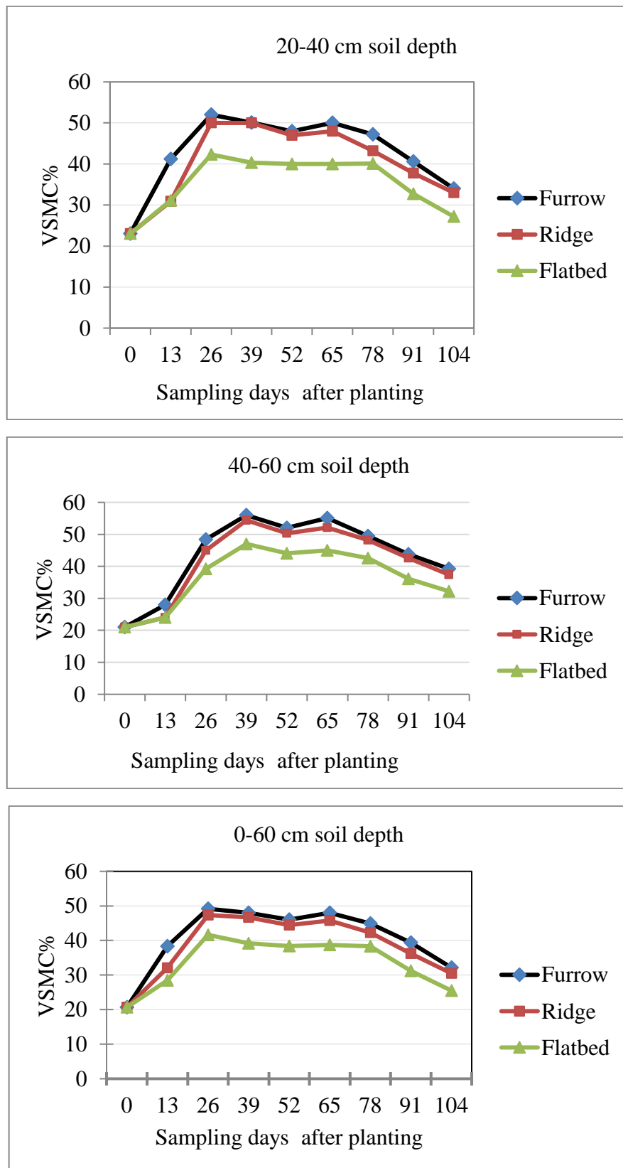
Fig. 3. Volumetric Soil Moisture Content (%VSMC) as Affected by Ridge, Furrow and Flatbed VSMC (%): Volumetric Soil Moisture Content; 0, 13, 26, 39, 52, 65, 78, 91, 104 are sampling days from planting (0) to harvest (104)
