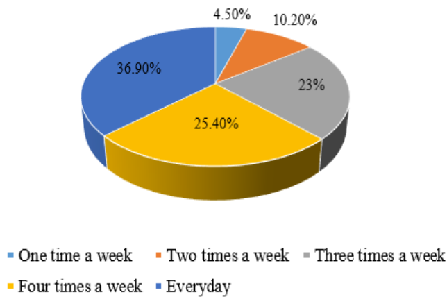
Fig. 1. Homework frequency
