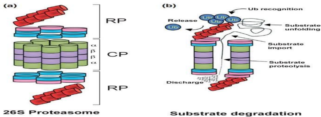
Fig. 2. Structure of 26S Proteasome [2]
