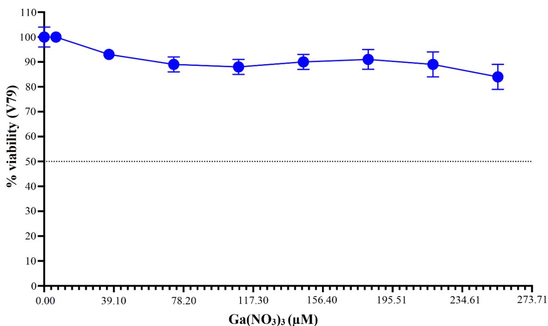
Fig. 3. V79 lineage cell viability in the presence of different concentrations of Ga(NO 3 ) 3 .
