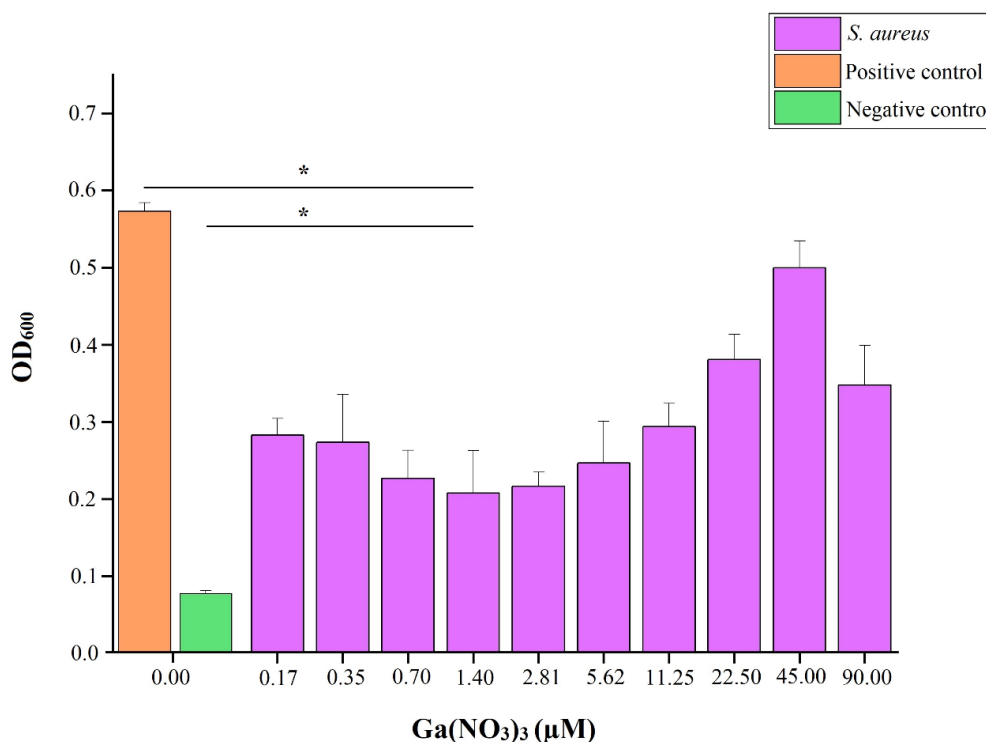
Fig. 1. Susceptibility of S. aureus treated with \text{Ga}(\text{NO}_3)_3 . Statistical significance between the absorbances data of positive and negative control against the pathogen data is indicated by an asterisk (* P=0.05 )
