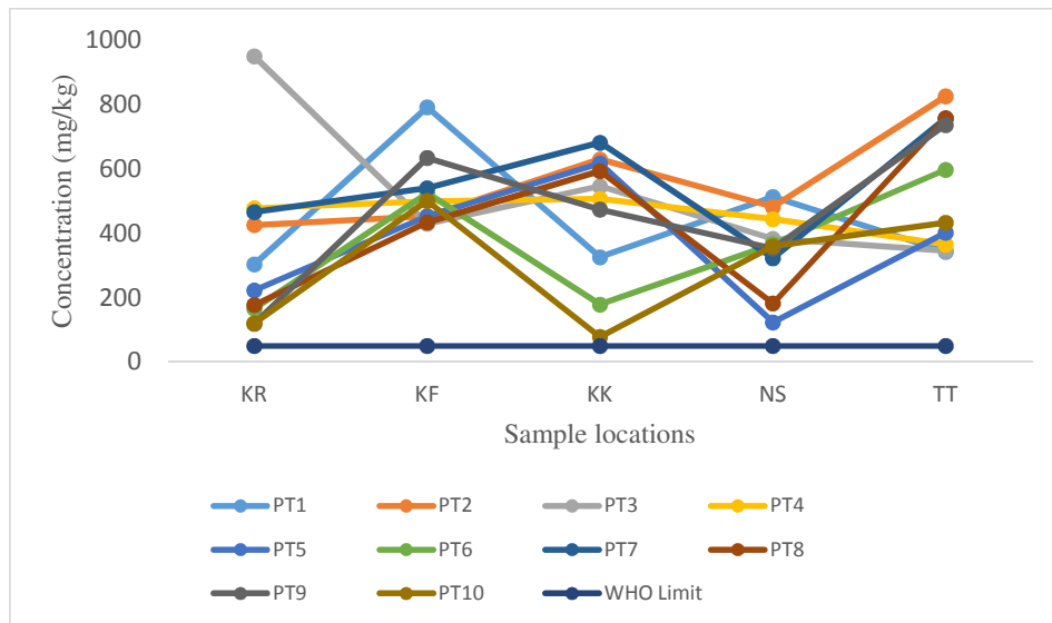
Fig. 7. Concentration of Nickel in swampy agricultural soil of Nasarawa west
