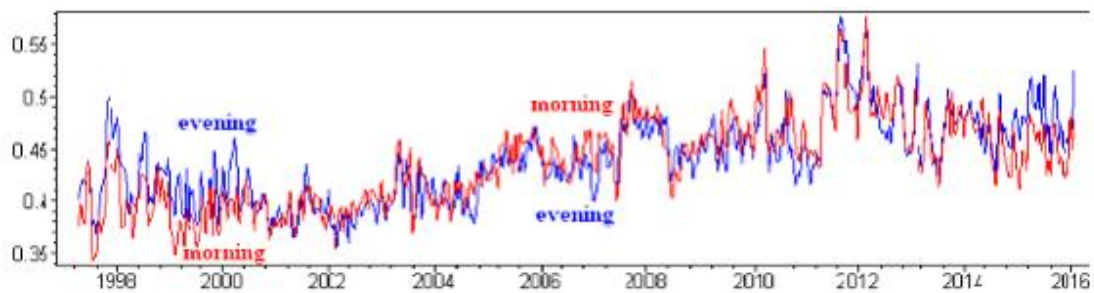
Fig. 5. The normalized pulse pressure, axis OX – year
