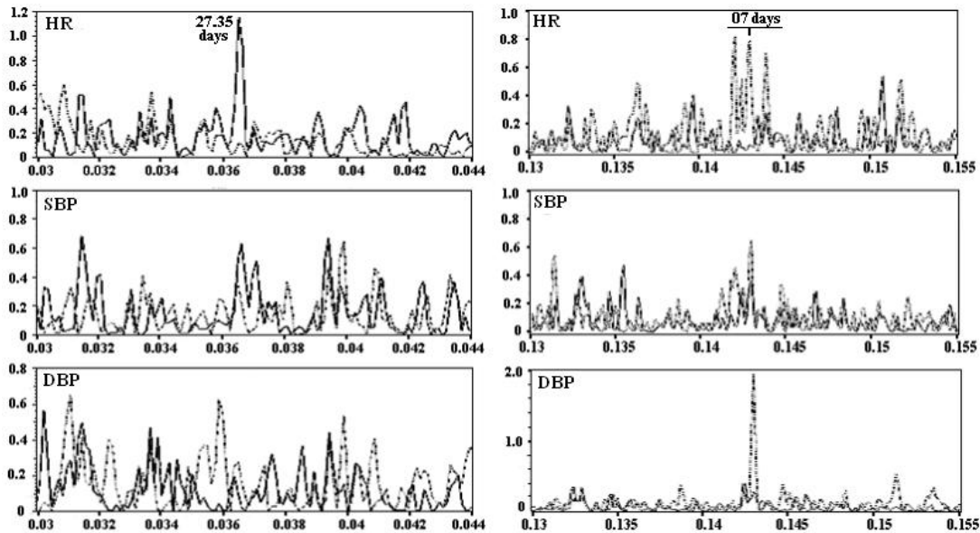
Fig. 4. Spectrum, neighborhood of 27-day (left) and 7-day (right) components: morning – dash line, evening – dot line
