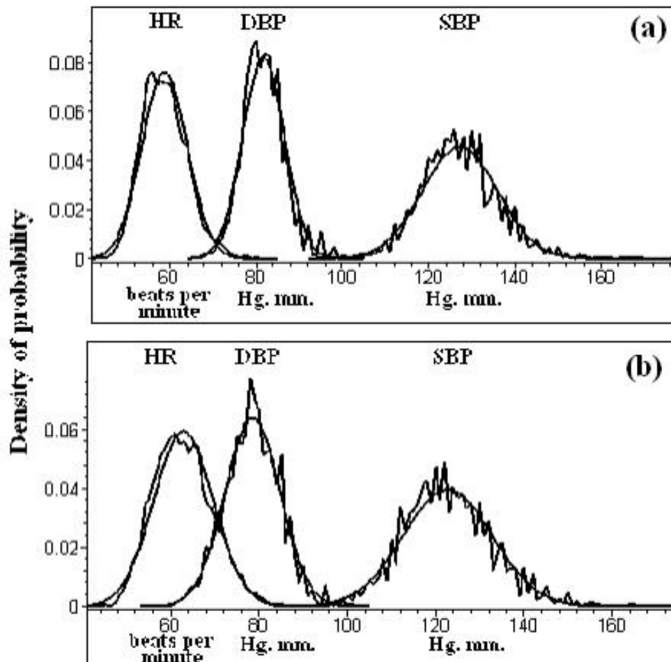
Fig. 2. Histograms: morning data (a), evening data (b)
