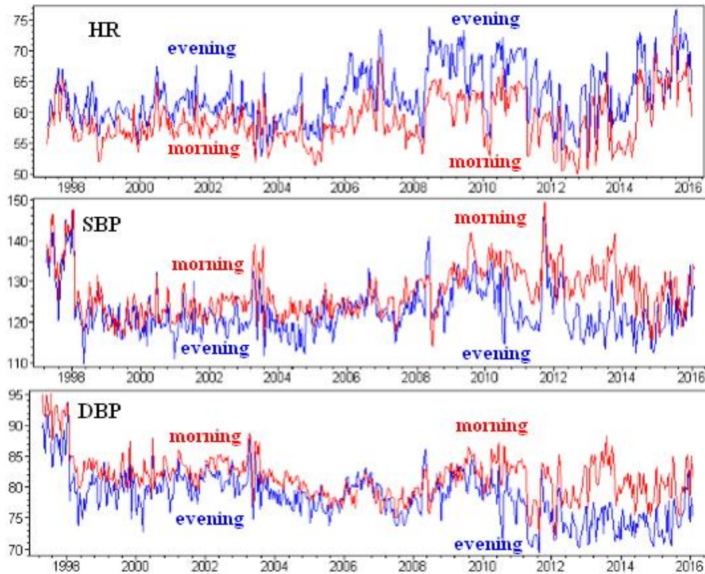
Fig. 1. Review of monitoring data: HR, SBP, DBP. Axis OX – year
