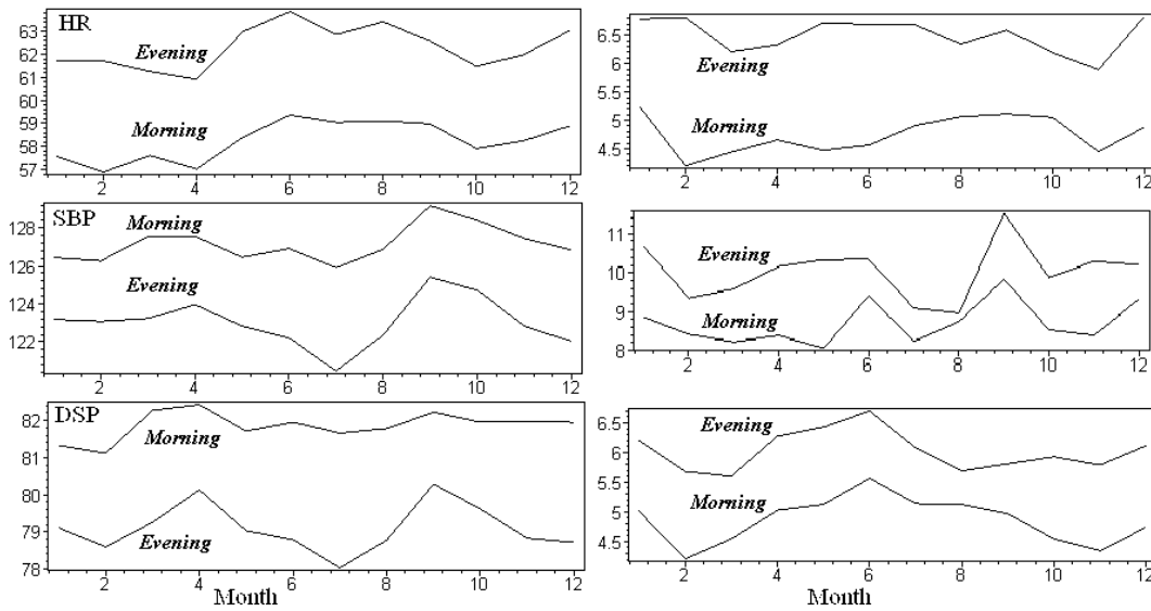
Fig. 3. Seasonal behavior of the HR, SBP, DBP (left side) and their variations (right side).
