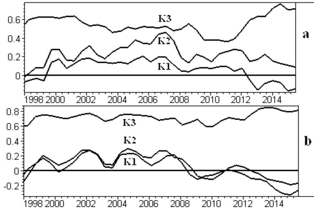
Fig. 6. Review of correlation series: morning data (a), evening data (b)
