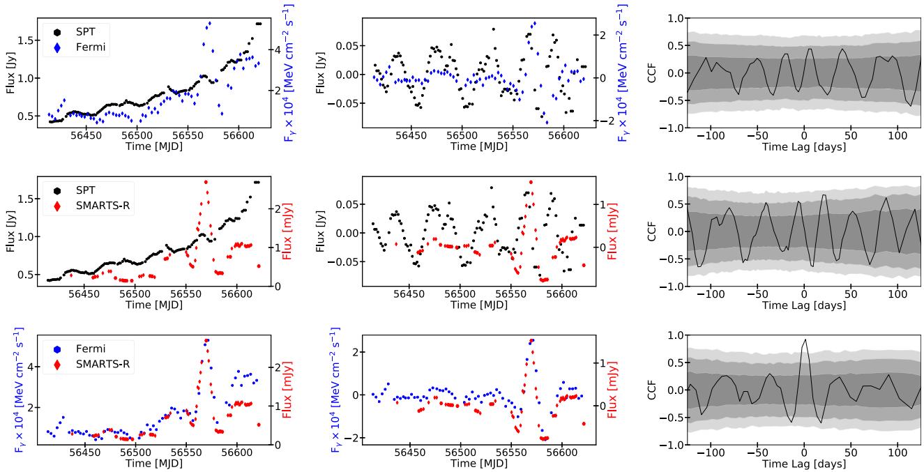
Figure 2. Year-1 boxcar-smoothed light curves (left column), smoothed and detrended light curves (middle column), and detrended CCFs (right column). The gray shaded regions represent the 1\sigma , 2\sigma , and 3\sigma contours of simulated CCFs.
