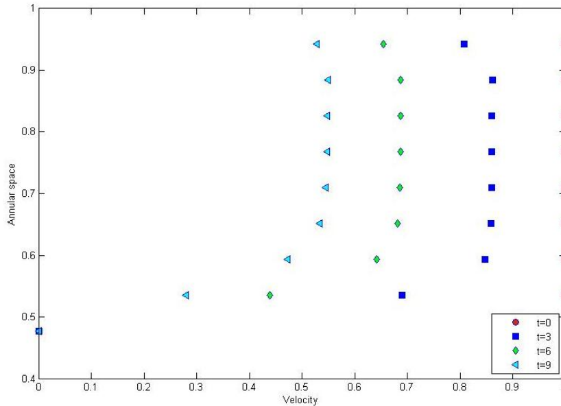
Fig. 7. Velocity profiles at different times for Case II when initially inner and outer pipes moving at same constant velocity at \eta = 0.477 (Velocity and annular space are non-dimensional)
