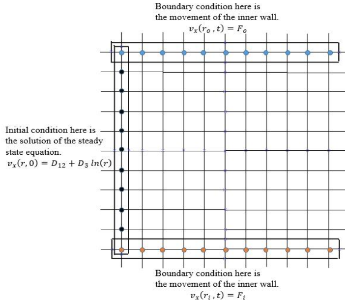
Fig. 2. Specifying initial and boundary conditions
