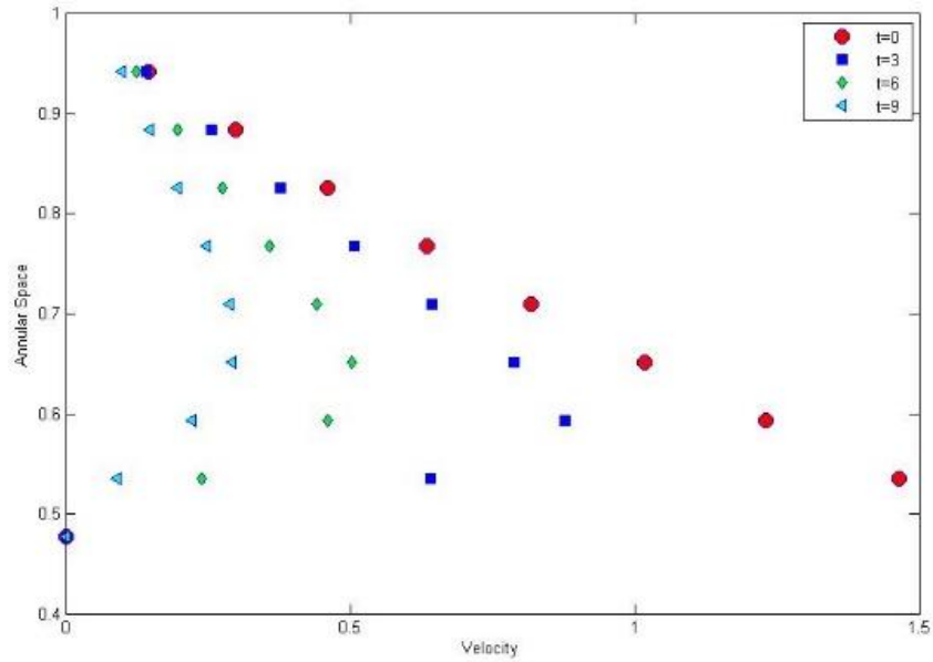
Fig. 5. Velocity profiles at different times for Case I when initially inner pipe moving at a constant velocity and outer pipe at rest at \eta = 0.477 (Velocity and annular space are non-dimensional)
