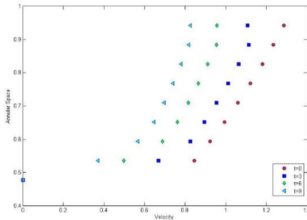
Fig. 10. Velocity profiles for abruptly stopped pipes at different times for Case III when V_o > V_i at \eta = 0.477 (Velocity and annular space are non-dimensional)
