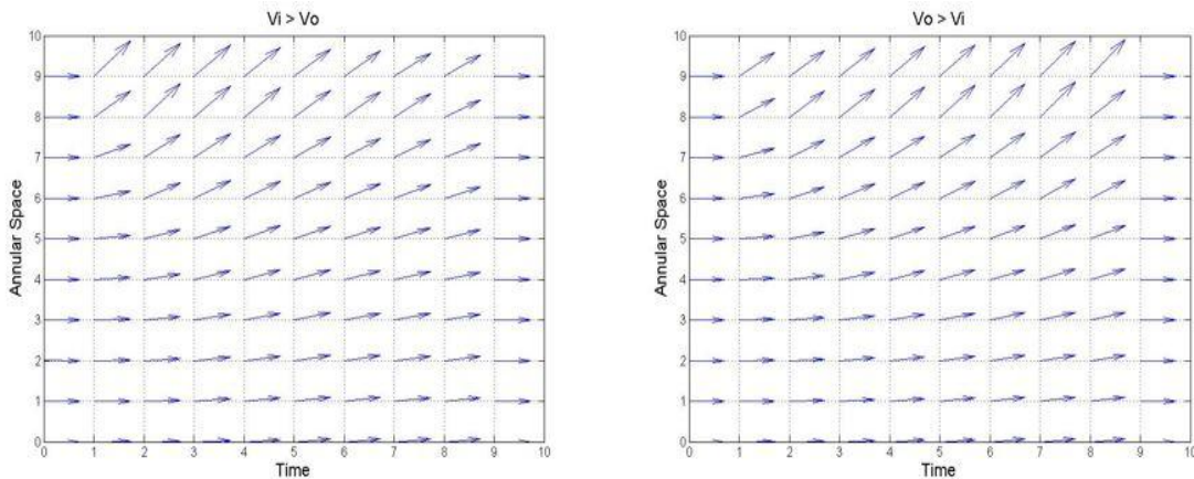
Fig. 8. Streamline of suddenly stopped axial Couette flow for Case III when inner and outer pipes in different constant velocities (Time and annular space are non-dimensional)
