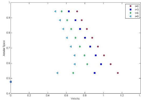
Fig. 9. Velocity profiles for abruptly stopped pipes at different times for Case III when V_i > V_o at \eta = 0.477 (Velocity and annular space are non-dimensional)
