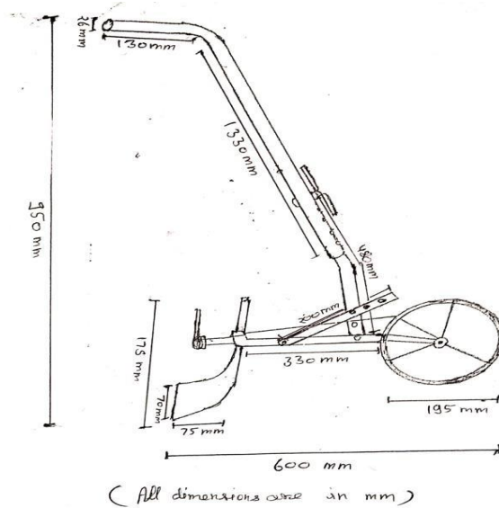
Fig. 1. Side view of hoe weeder
