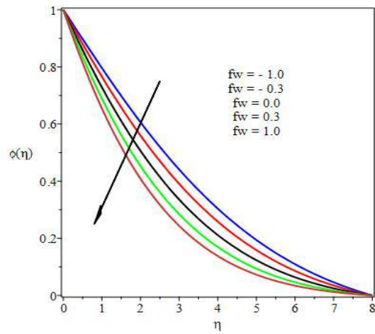
Fig. 14. Concentration profiles for different values of fw
