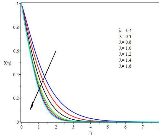
Fig. 10. Temperature profiles for different values of \lambda
