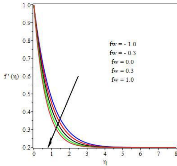
Fig. 12. Velocity profiles for different values of fw
