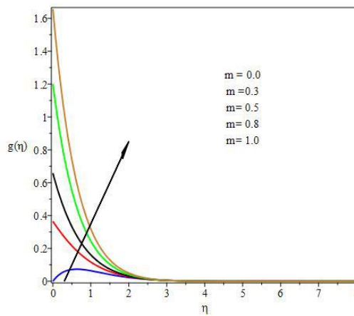
Fig. 19. Microrotation profiles for different values of m
