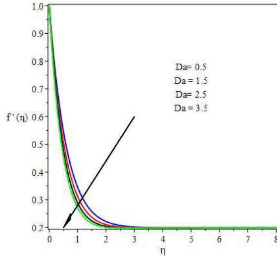
Fig. 7. Velocity profiles for different values of Da
