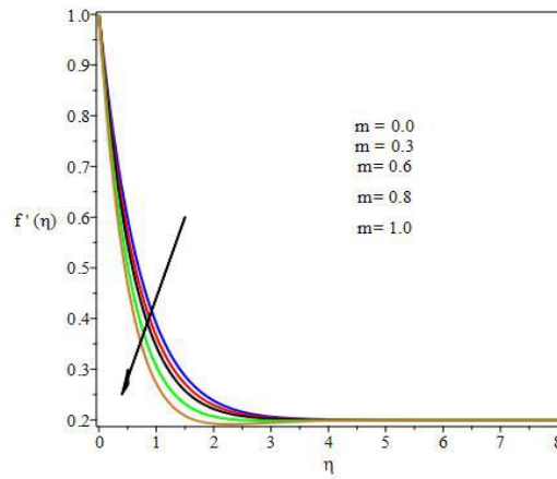
Fig. 18. Velocity profiles for different values of m
