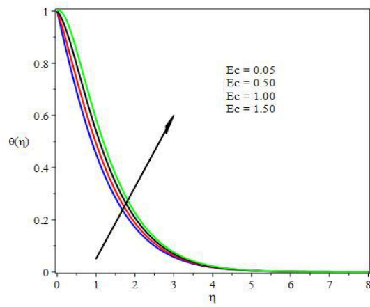
Fig. 15. Temperature profiles for different values of Ec
