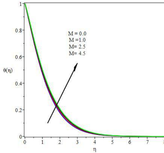
Fig. 3. Temperature profiles for different values of M
