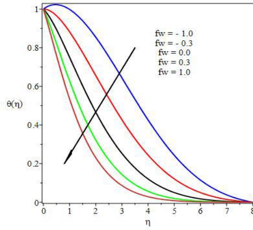
Fig. 13. Temperature profiles for different values of fw
