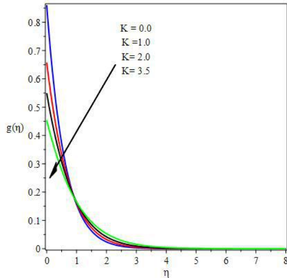
Fig. 6. Microrotation profiles for different values of K
