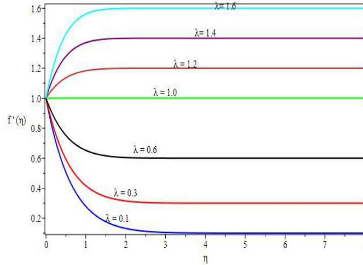
Fig. 9. Velocity profiles for different values of \lambda
