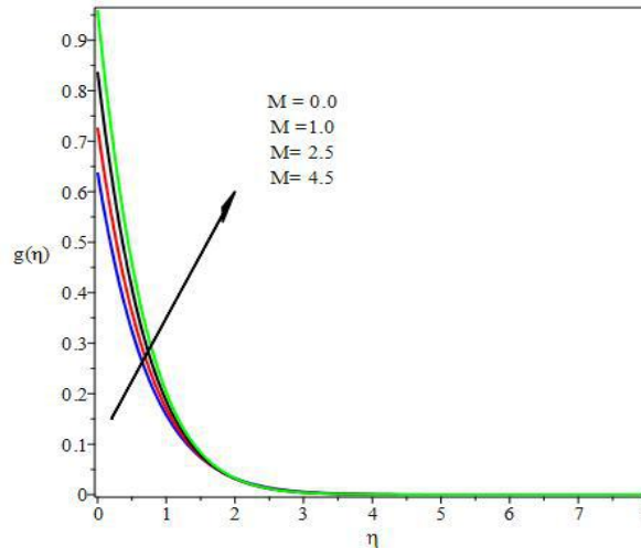
Fig. 4. Microrotation profiles for different values of M
