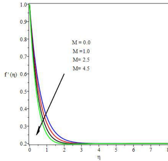
Fig. 2. Velocity profiles for different values of M
