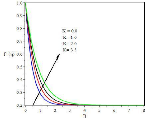
Fig. 5. Velocity profiles for different values of K
