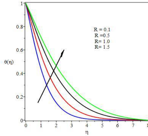
Fig. 16. Temperature profiles for different values of R
