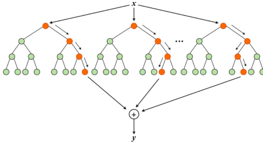
Fig. 6. Architecture of Random Forest
