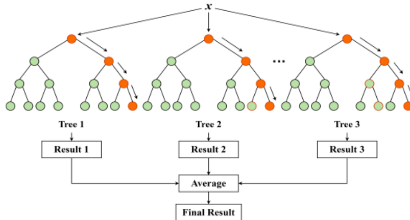
Fig. 7. Architecture of XGBoost
