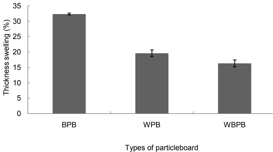
Fig. 6. Thickness swelling of three types of particleboard
