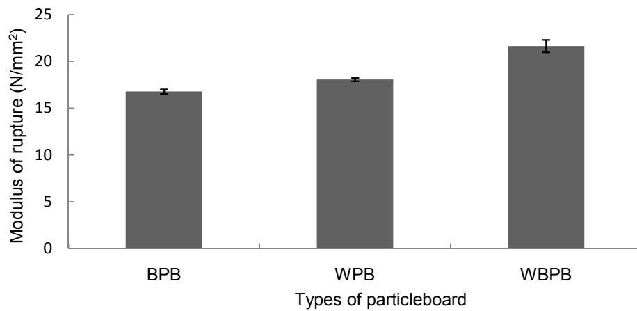
Fig. 3. Modulus of rupture (MOR) of three types of particleboard
