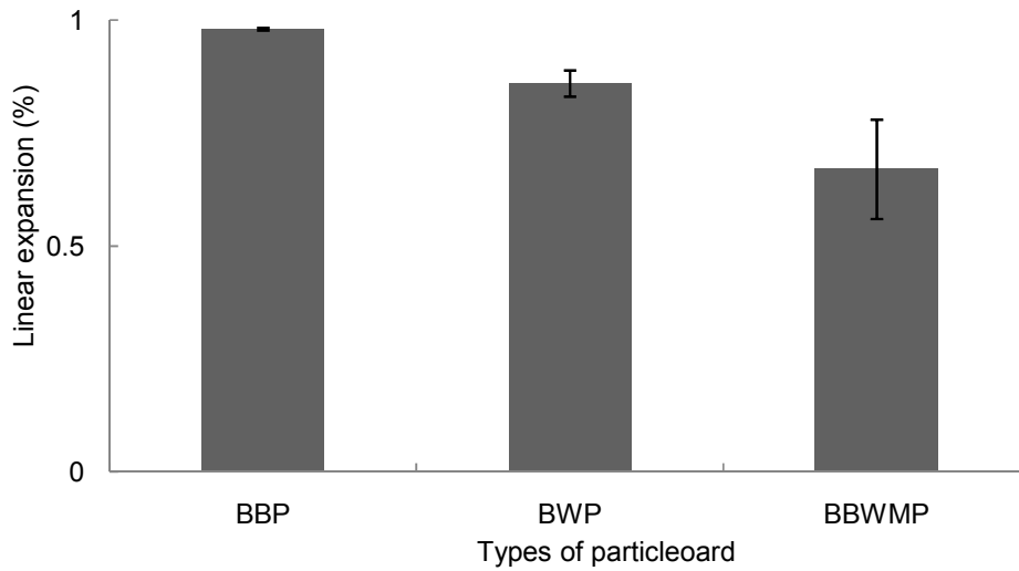
Fig. 5. Linear expansion of three types of particleboard
