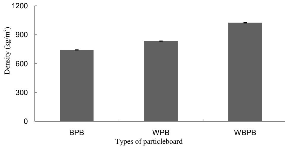
Fig. 1. Density of three types of particleboard
